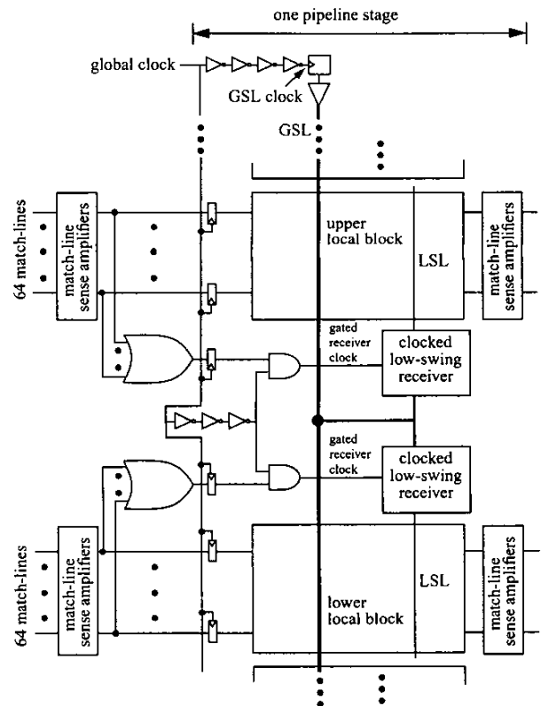
Fig. 4. Hierarchical search-line architecture. Low-swing global search-lines drive the full height of the CAM macro. Full-swing local search-lines span the height of a local block. The clocked low-swing receivers are enabled only when the previous local block has at least one match, saving power.
