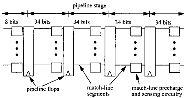
Fig. 3. Pipelined match-line architecture. The match-lines are broken into five match-line segments. A segment is activated only if there is a match in the previous segment.
