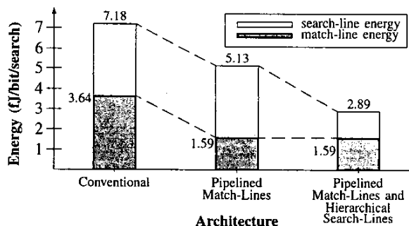
Fig. 2. CAM search cycle energy dissipation for the conventional architecture, pipelined match-lines, and pipelined match-lines with hierarchical search-lines.
