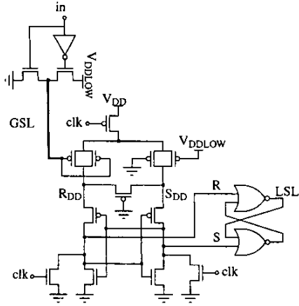
Fig. 5. Low-swing receiver.
