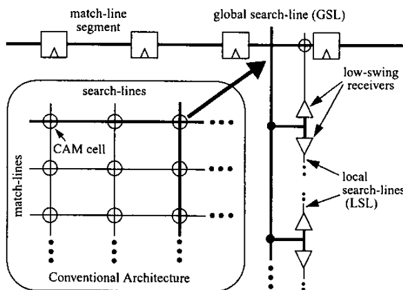
Fig. 1. CAM architecture with pipelined match-lines and hierarchical search-lines.
