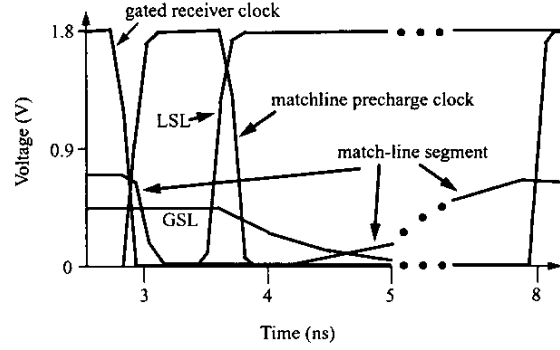
Fig. 6. Signal waveforms for a full search operation. The cycle time is dominated by the charging of the match-line segments. A portion of the cycle time, showing the rising match-line, has been removed to simplify the figure.
