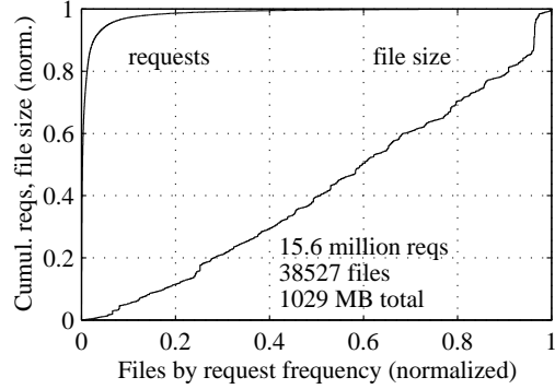
Figure 6: IBM Trace
