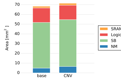
Fig. 11: Area Breakdown
