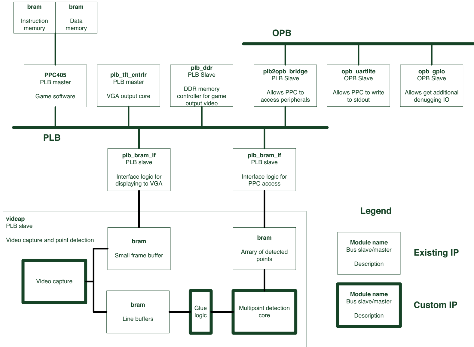
Figure 1 Block diagram of the project
