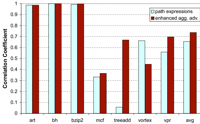
Figure 9: Comparing accuracy of path expression and aggregate advantage frameworks
