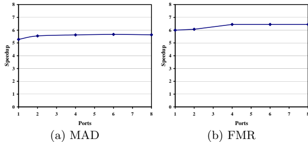
Figure 16: Impact of the number of memory ports on the speedup at 8 processors.
