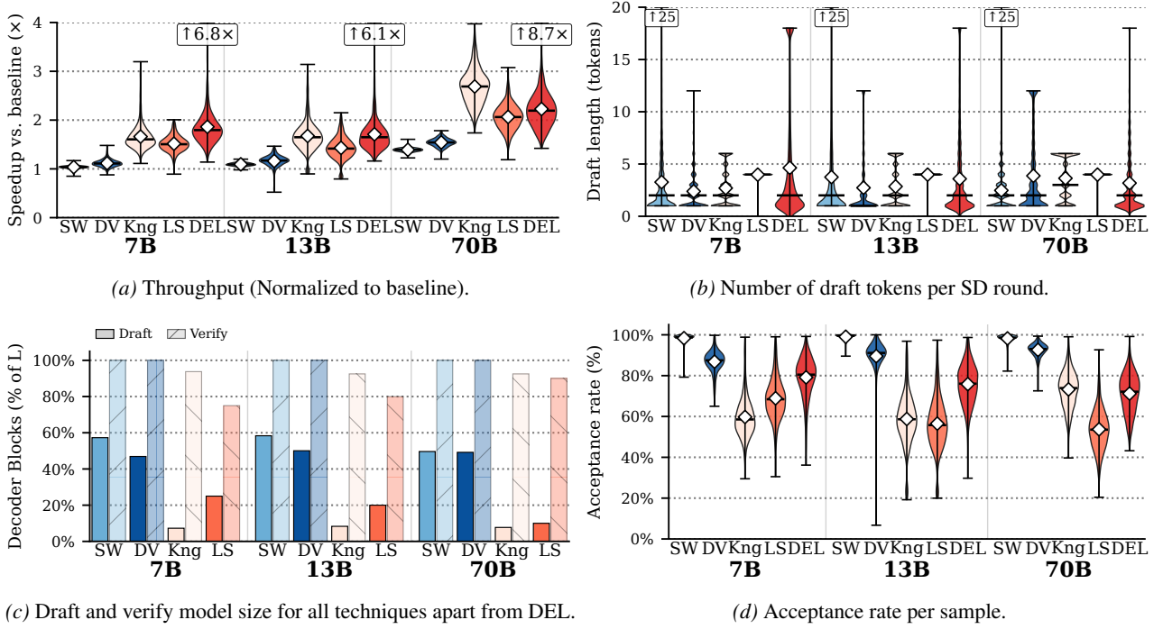
Figure 12. Results for layerskip-llama-2 7B, 13B &amp; 70B models for the GSM 8k dataset.
