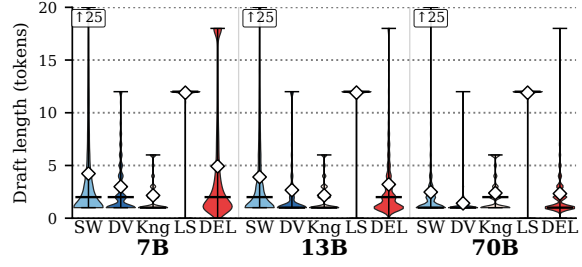
(b) Number of draft tokens per SD round.
