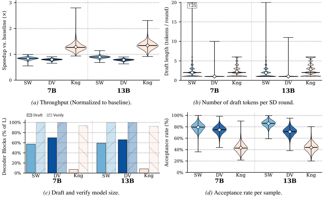
Figure 23. Results for Vicuna-v1.3 7B &amp; 13B on GSM8K.
