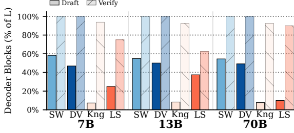
(c) Draft and verify model size (Appendix A) for all techniques apart from DEL, normalized to the total number of decoder blocks. Verify size reflects only the blocks executed during verification.
