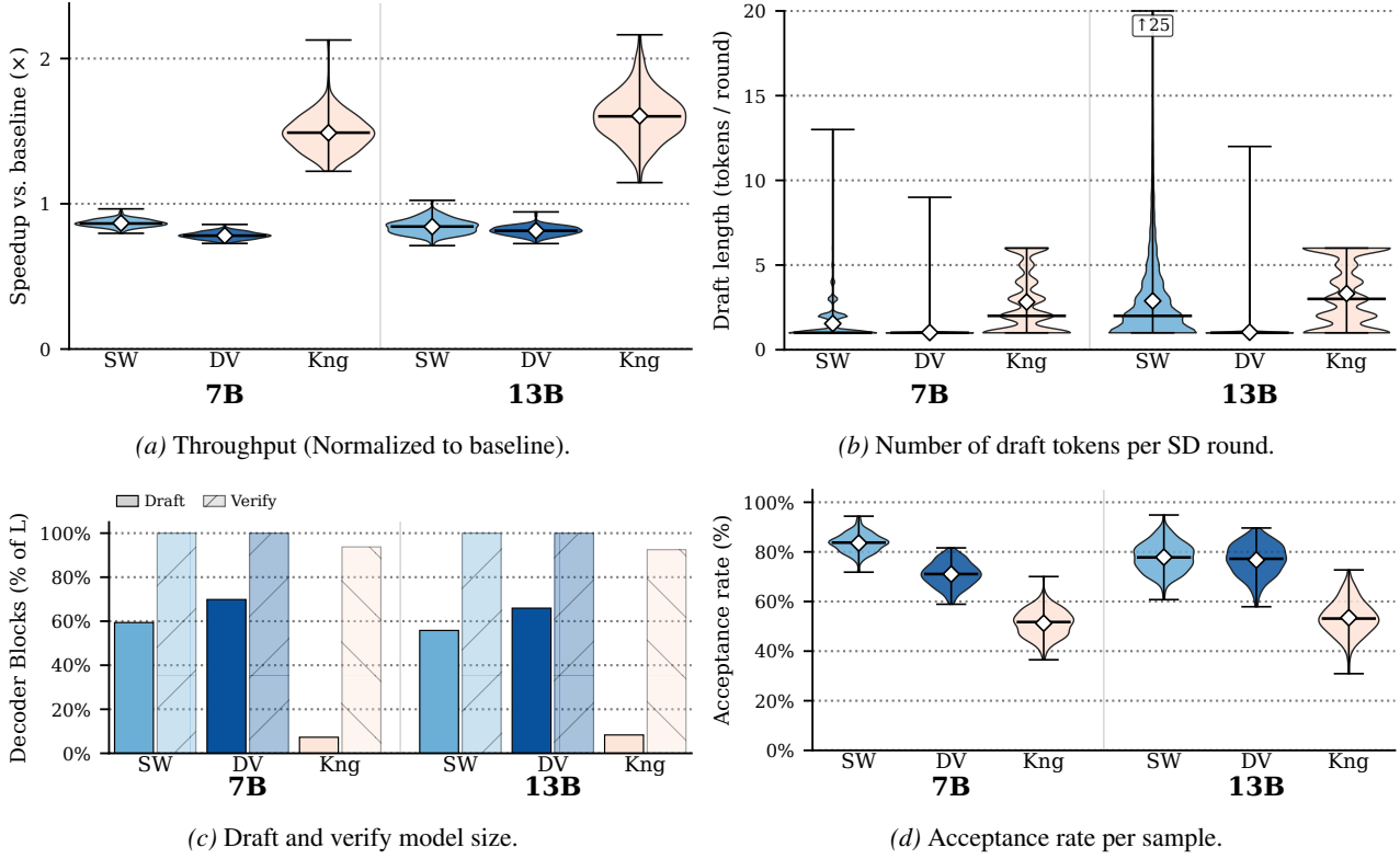
Figure 22. Results for Vicuna-v1.3 7B &amp; 13B on HumanEval.
