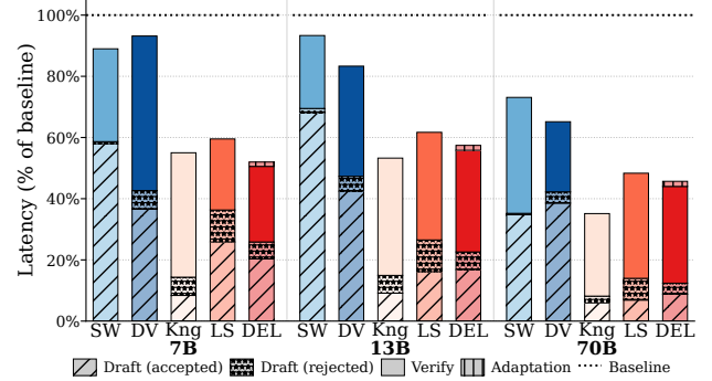
Figure 4. Latency breakdown, normalized to the baseline for LayerSkip-llama-2 models on HumanEval . ‘Adaptation’ segment represents DEL ’s per-round reconfiguration overhead.
