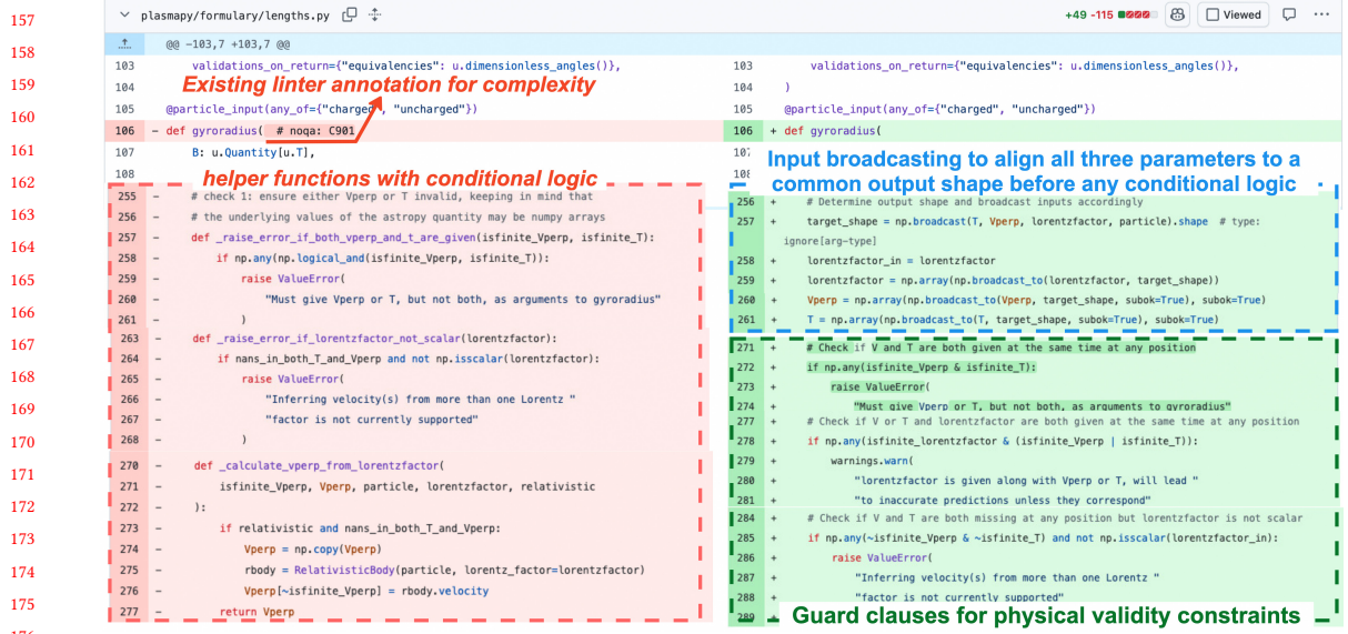
Fig. 1. Motivating example from PlasmaPy/PlasmaPy PR#2542. Left Side (Before) and Right Side (After). Nested control flow (dashed red box) is replaced by input broadcasting (dashed blue box) and flat guard clauses (dashed green box).
